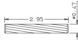
Dowel
