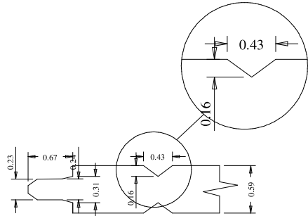
Panel Profile
